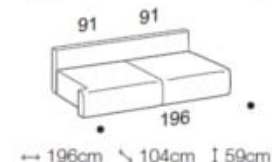
Cod. (&lt;-) E-BL100MS - E-BL100MD (-&gt;)
